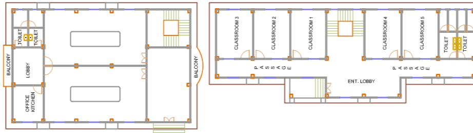
PLAN OF PRINCIPAL QTR BLOCK & ADDITIONAL COURSES BLOCK
